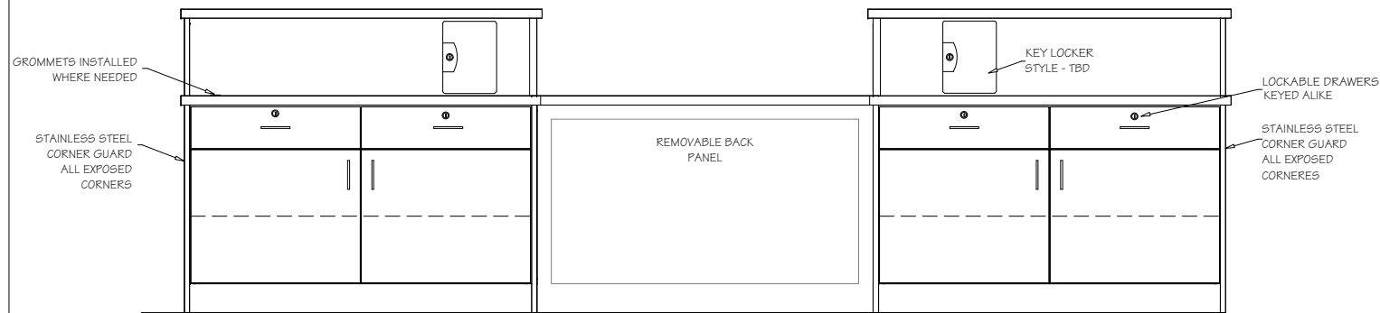
C Employee Side Scale: 1/2=1
