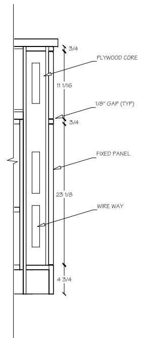
G Wall Detail Scale: 3/4=1
