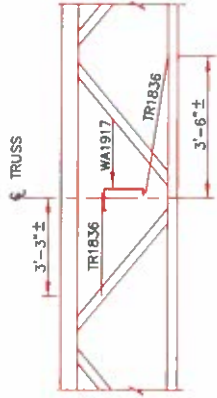
BRACKET BRACE DETAIL (VIEW FROM INSIDE)
